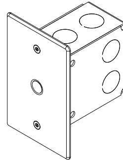
VIEW WITH JBOX - JBOX PROVIDED BY OTHERS
