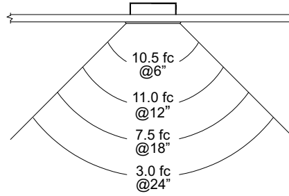
Footcandle Performance On the Floor - Top View ITL Test: 89228
