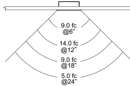
Footcandle Performance On the Floor - Top View
