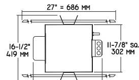
Plan View A
