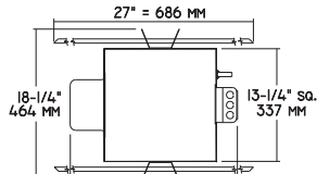
Plan View B
