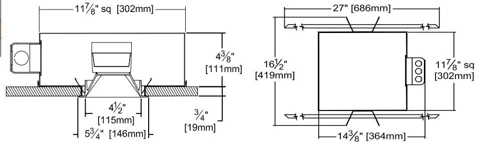
Ceiling Cut-out 5 1/4" Sq.
