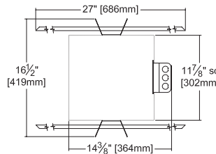
Ceiling Cut-out 9" Dia.
