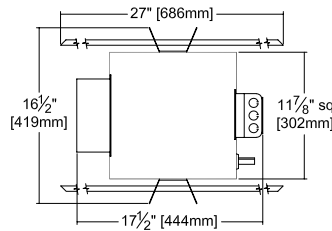
Ceiling Cut-out 10 1/4" Dia.
