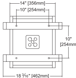
Ceiling Cut-out 13" x 15 1/2"
