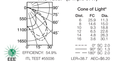
VRS-12027 (2 Triple 57W)
