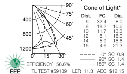
VRR-10058 (150 Watt)
