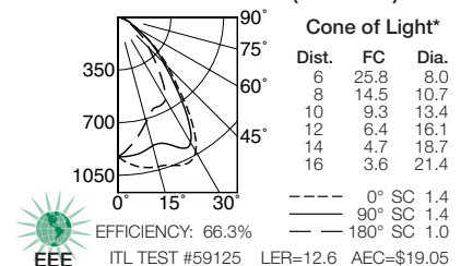
VRR-10058 (150 Watt)
