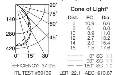
VRR-07001 (1 Triple 26W)
