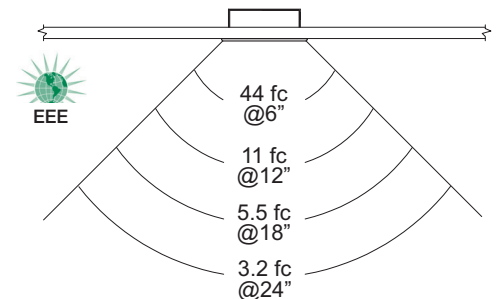
Footcandle Performance Opposite Fixture Installed Top View
