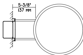
Representative View: With optional wall bracket (Option -WB)
