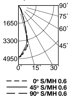
RS30963 (120W Flood Shown)
