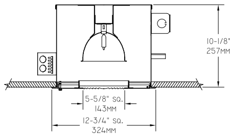
Ceiling Cut-out 12 1/4" Sq.
