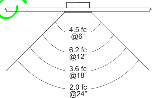
Footcandle Performance On the Floor - Top View (Installed 14" above finished floor.)
