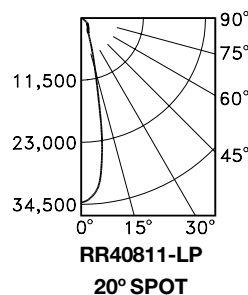
CP Distribution (Assumes use in vertical position)
