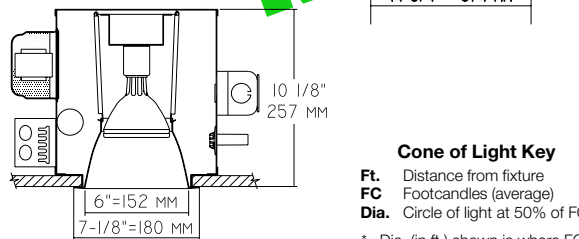
RR40626 (10° Narrow Spot Shown)
