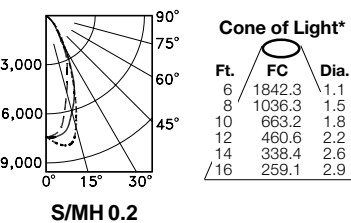
RR40626 (10° Narrow Spot Shown)
