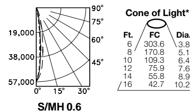
RR40626 (40° Medium Flood Shown)
