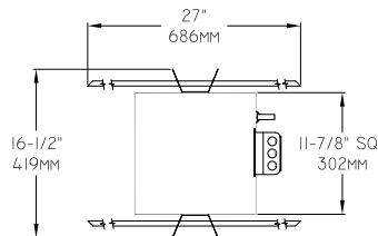
Ceiling Cut-out 6 1/2"
