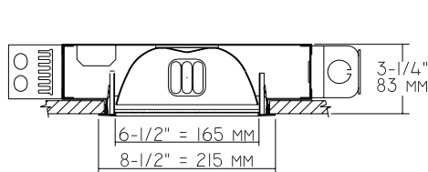
Ceiling Cut-out 8"
