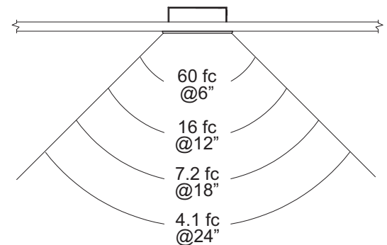
Footcandle Performance Opposite Fixture Installed Top View
