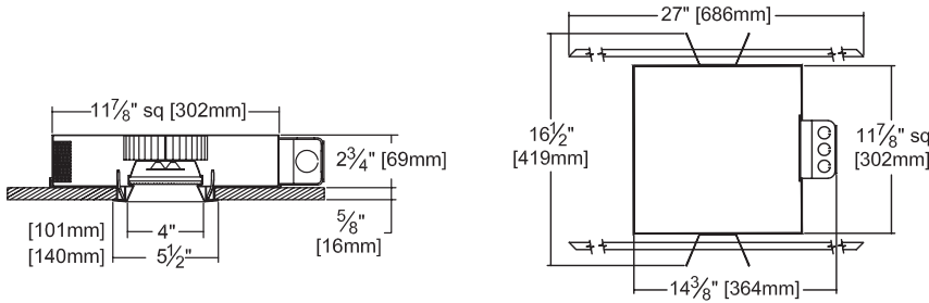
Ceiling Cut-out 5" Dia.
