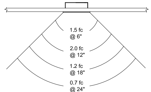
Footcandle Performance On the Floor - Top View (Installed 14" above finished floor.)
