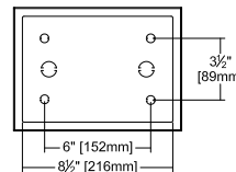
Housing KO's
