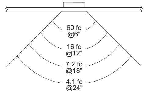
Footcandle Performance Opposite Fixture Installed Top View
