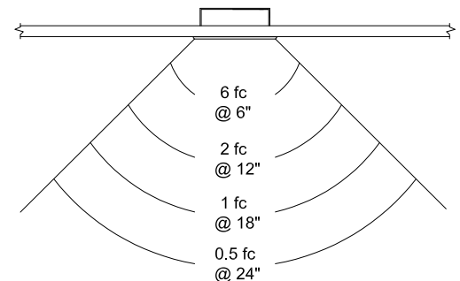
Footcandle Performance Opposite Fixture Installed Top View
