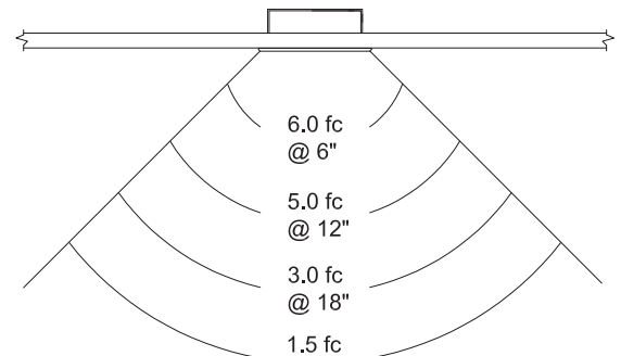
Footcandle Performance On the Floor - Top View (Installed 14" above finished floor)
