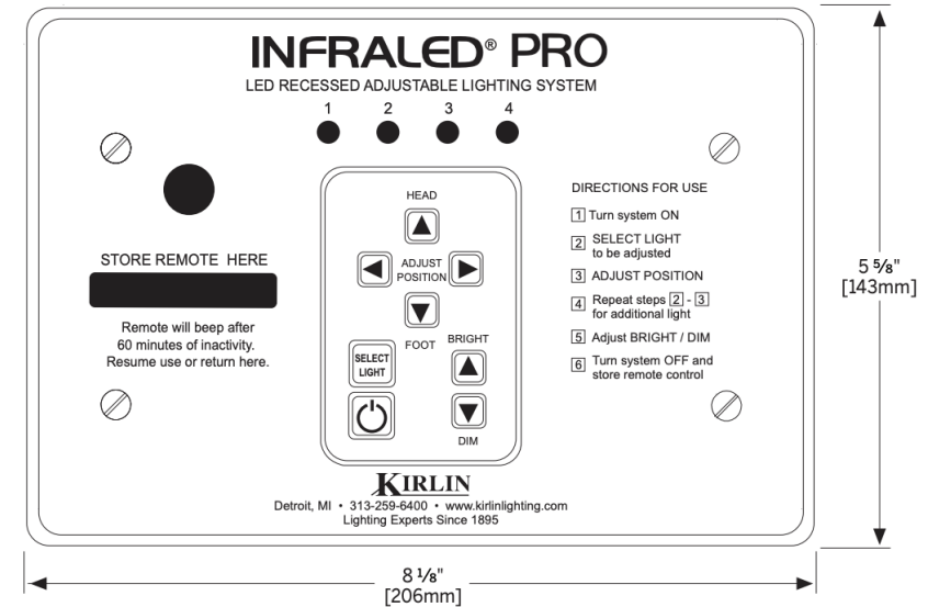
Wall Control Panel (PRO-WALLC)
