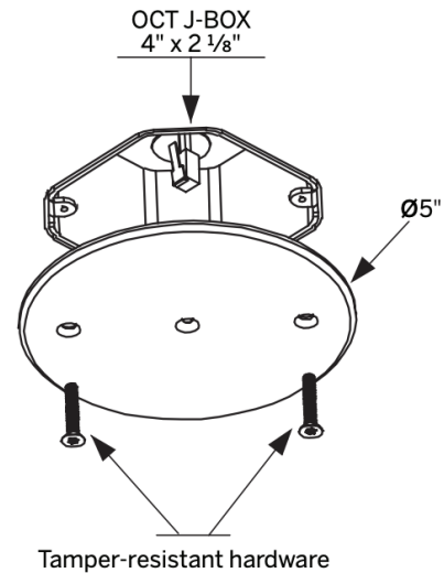
Ceiling Mounted Infrared Sensor (PRV-SENSR)
