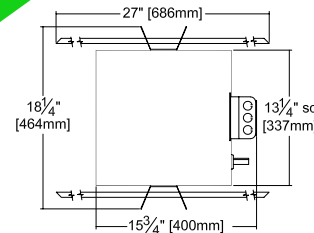
Ceiling Cut-out 9" Dia.
