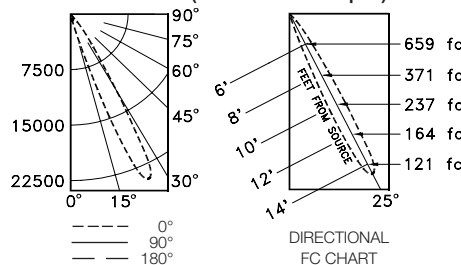
IRR-07098 (120W Narrow Spot)
