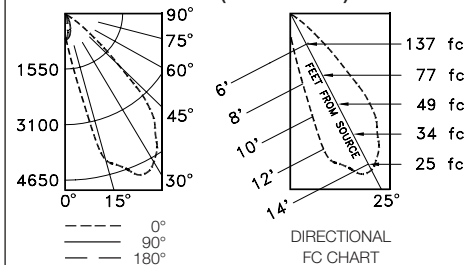
IRR-07098 (120W Flood)
