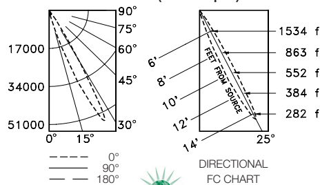
IRR-07096 (250W Spot)
