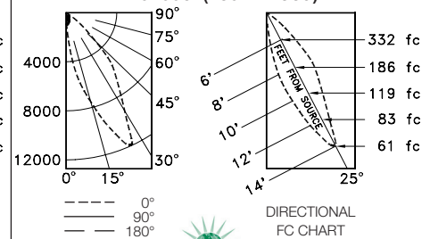
IRR-07096 (250W Flood)
