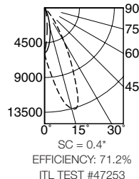
IRR-07062 (Clear Lamp)
