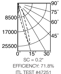
IRR-07062-28 (Frosted Lamp)
