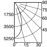
IRR-07058-15 (Frosted Lamp)
