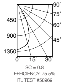
IRR-04008 (50 Watt VWFL60)
