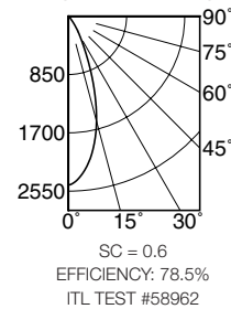
IRR-04008 (50 Watt FL35)
