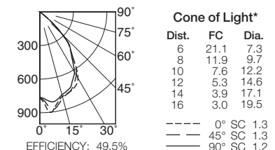
FSR-06046 (1 Triple 32W)
