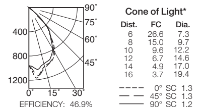
FSR-06046 (1 Triple 42W)
