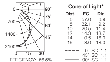
FRS-10109 (2 Triple 57W)
